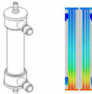
Blood Cardioplegia Device
