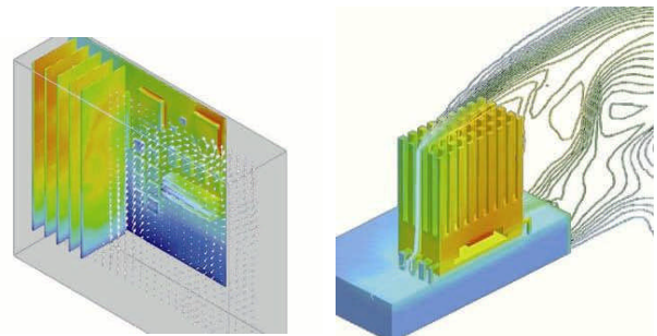
Electronics Cooling
